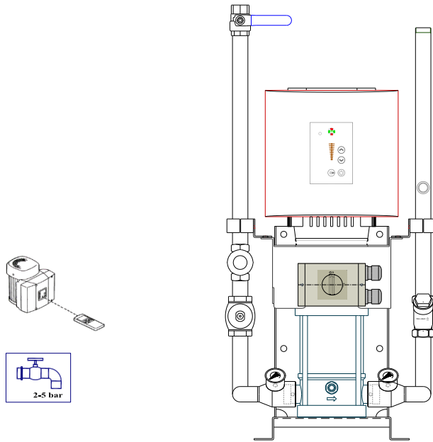
PumpSet Freq. 25- 30 IE5. Vertical in/out
